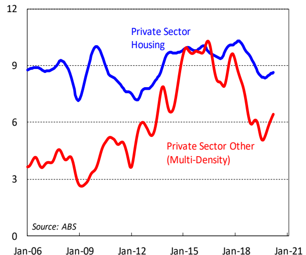
Number of Building Approvals (In Thousands, Trend Data)
